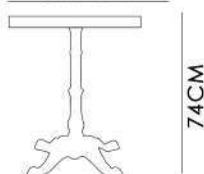
Telsa, Ø40 cm, height 74cm
